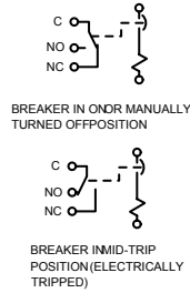
Mid-Trip Handle Positions
