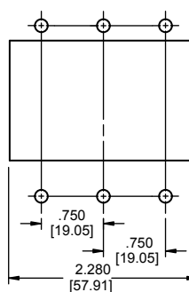
Two Pole*
