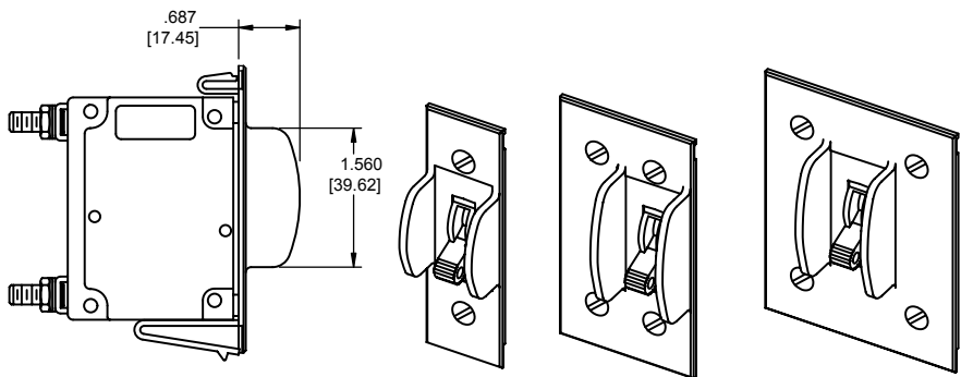
Panel Mounting Options
