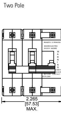
Two Pole*
