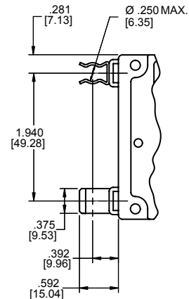
Clip Terminal
