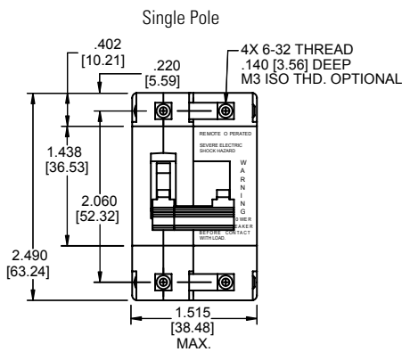
Panel Mounting Details Single Pole
