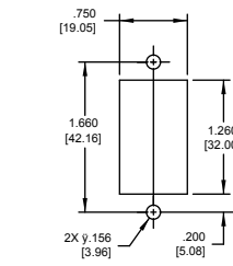
Panel Mounting Detail Mounting Detail Tolerance: ±.005 [.13] unless noted
