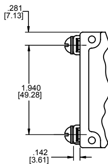
Screw Terminal
