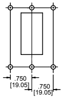
Mounting Detail*
