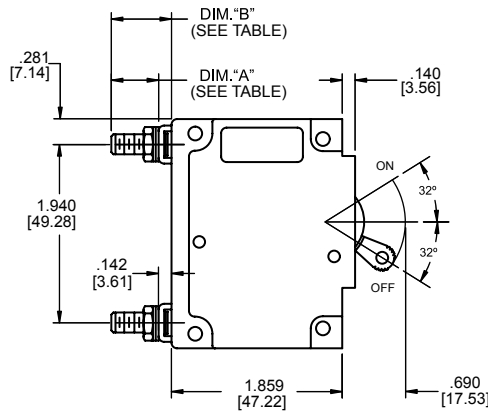
Single Pole, Standard Stud Terminal
